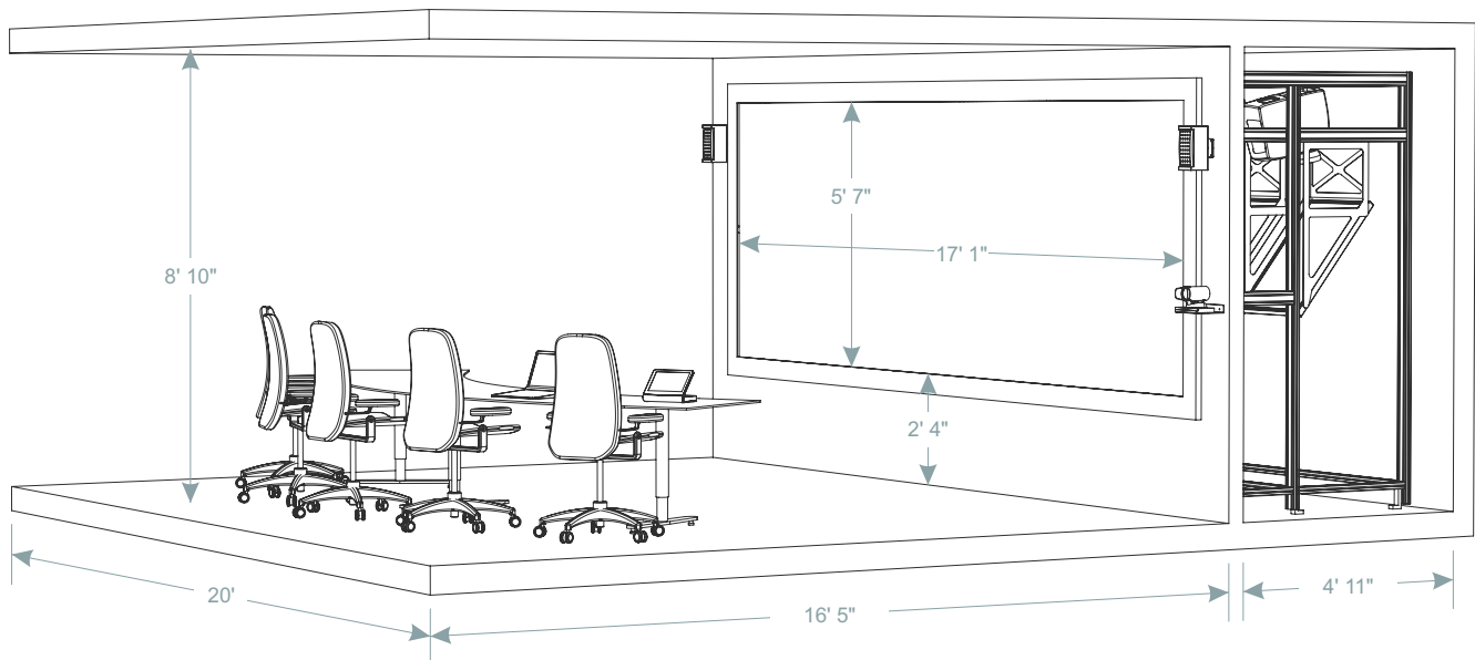
Dimensions indicate a typical installation and may be changed to match customer requirements.
